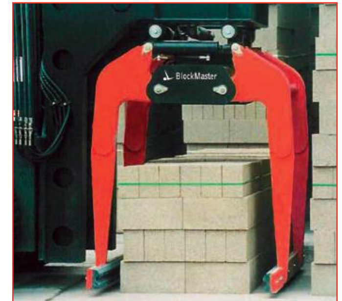
BC30 Twin Overhead Block Clamp
